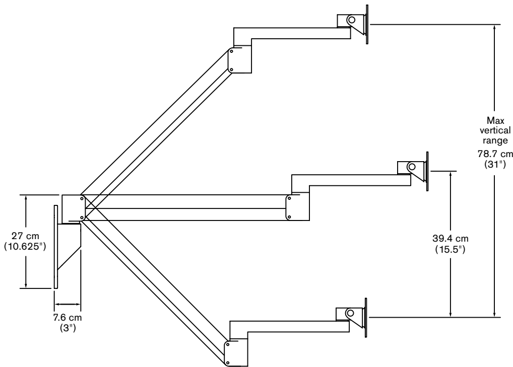
SIDE VIEW Vertical Range
