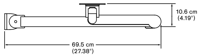
TOP VIEW Arm Folded
